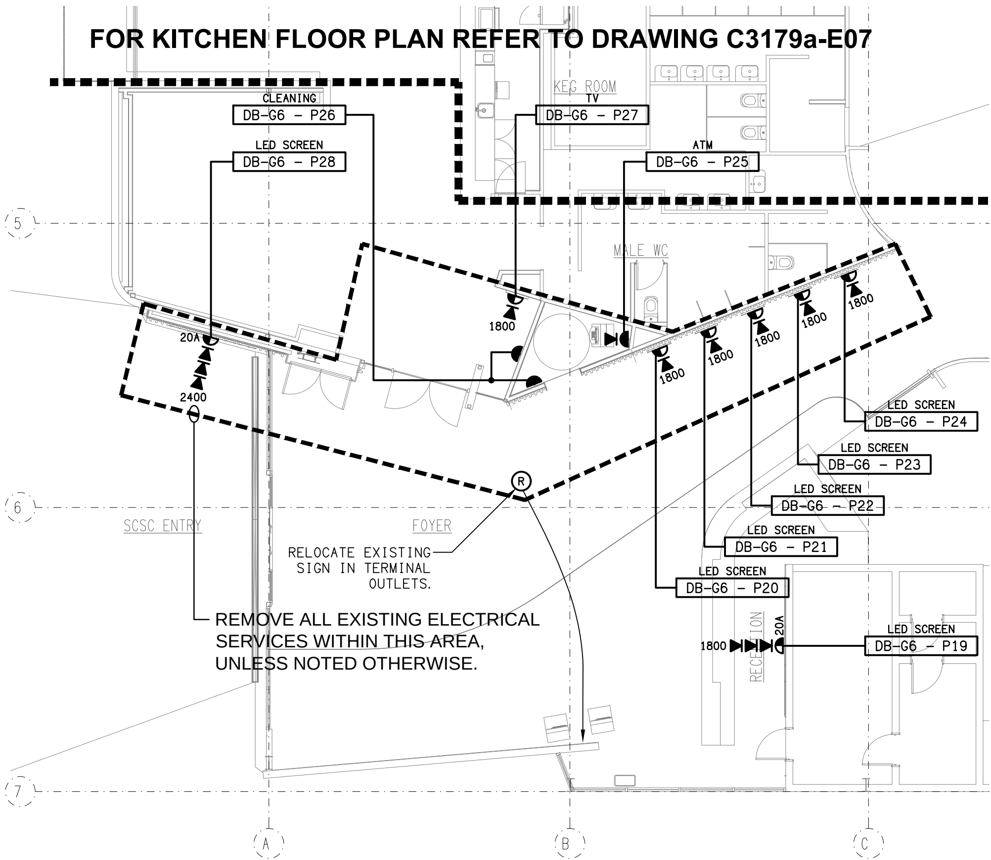
FLOOR PLAN PROPOSED FOYER SCALE 1: 100
