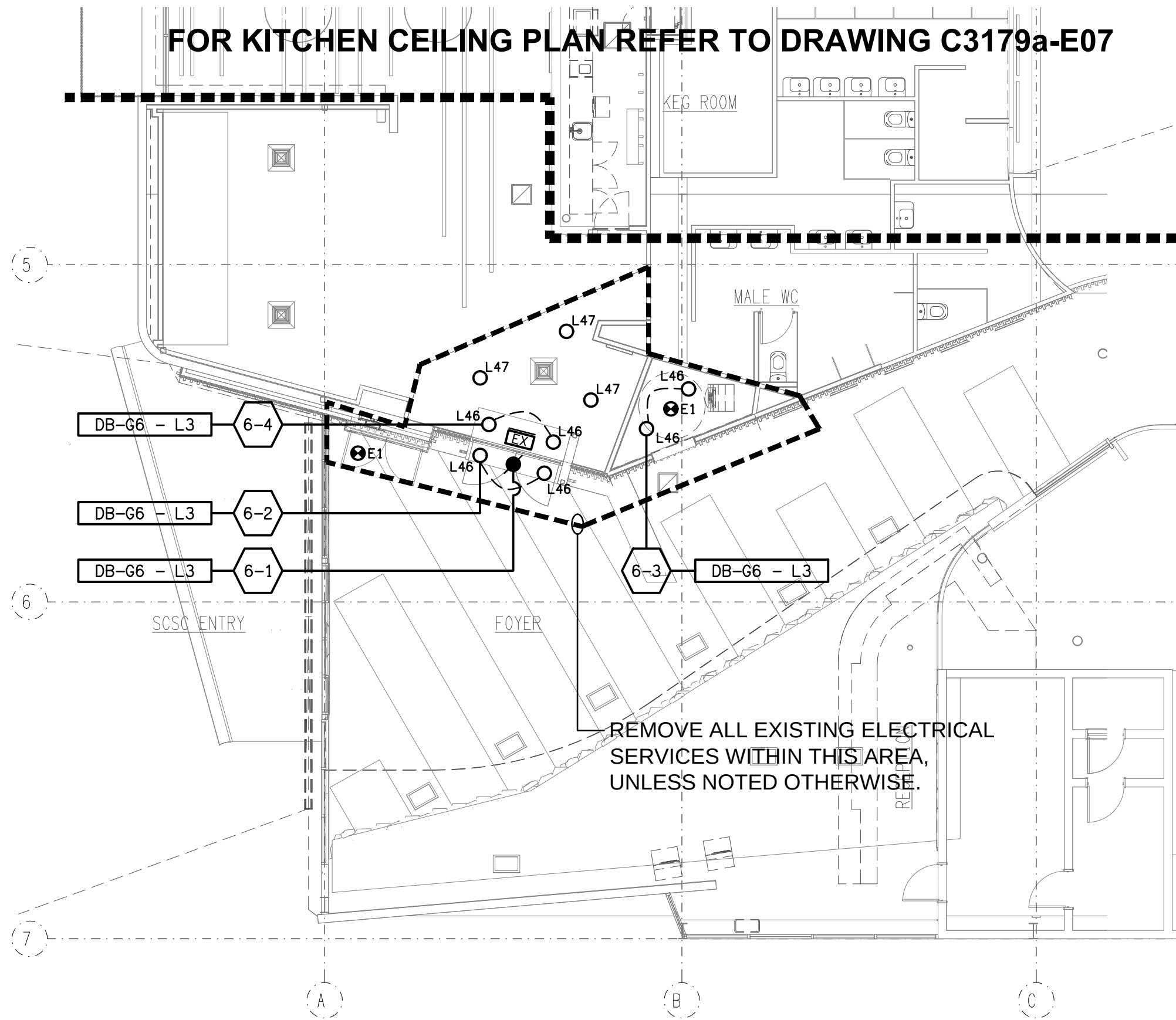
REFLECTED CEILING PLAN PROPOSED FOYER SCALE 1: 100
